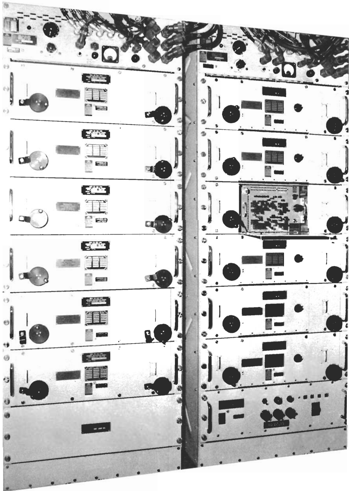
C.A.W. OUTFITS EBA1 & EBA2 IN CABINET OUTFITS YBU FIG 11.4
